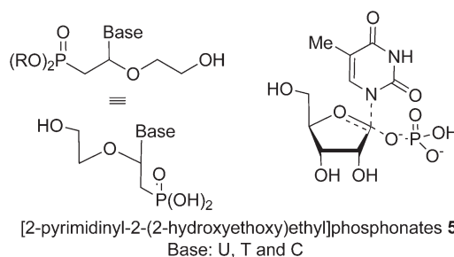
Fig. 2 Targeted acyclic nucleoside analogues and transition state derivative of thymidine phosphorylase.
